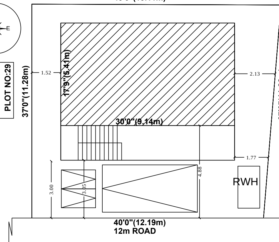
SITE PLAN
