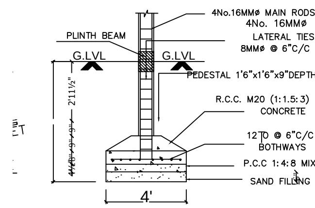
FOUNDATION DETAIL
