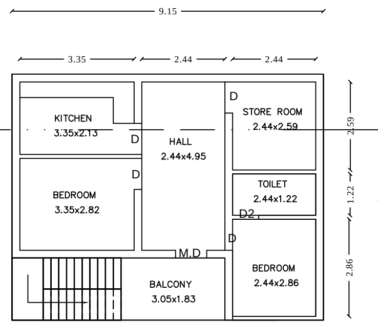
TYPICAL FIRST AND SECOND FLOOR
