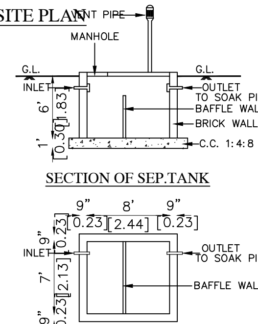
PLAN SEPTIC. TANK
