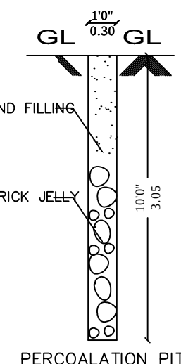
RAIN WATER HARVESTING SYSTEM
