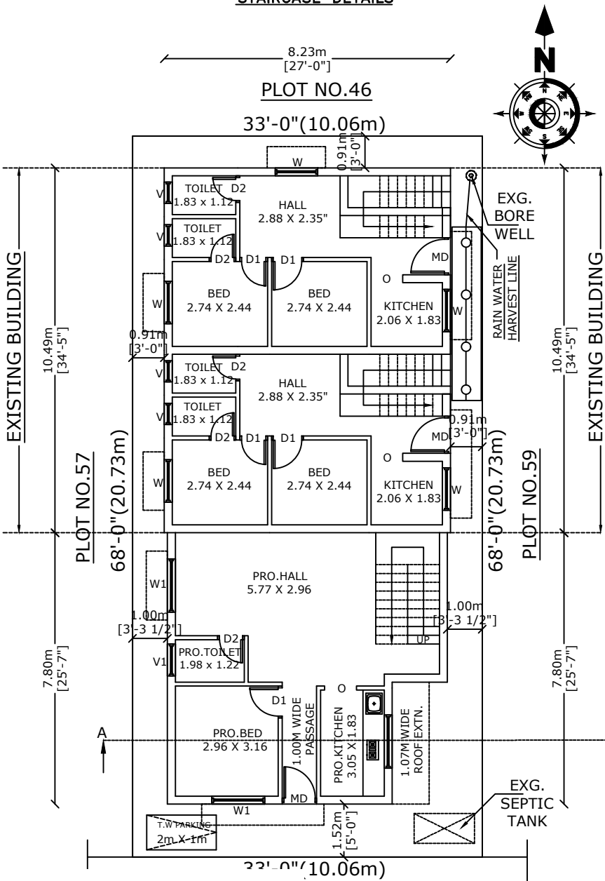
EXISTING BUILDING FLOOR PLAN
