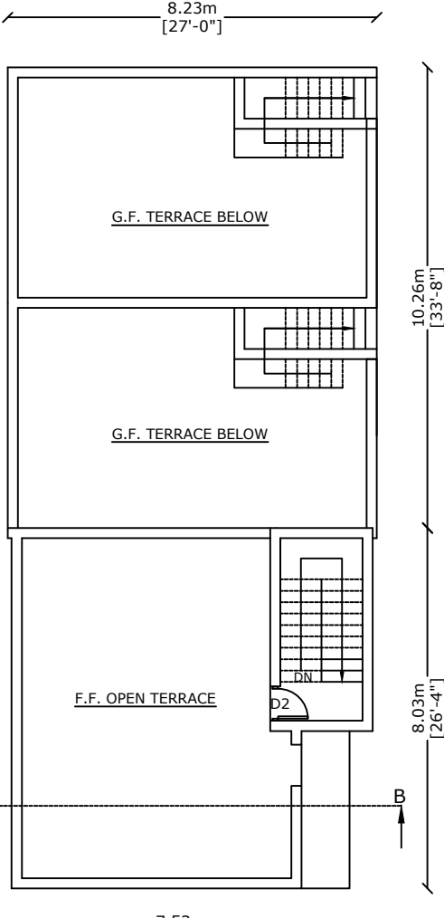
PRO. TERRACE FLOOR PLAN
