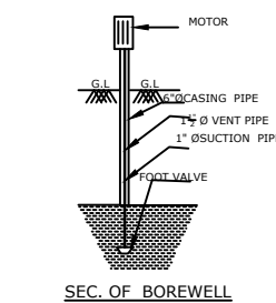
SEC. OF BOREWELL
