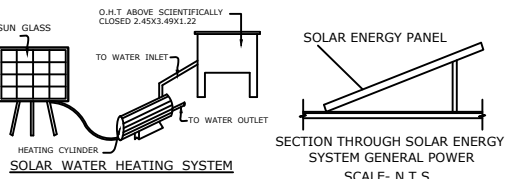
SOLAR WATER HEATING SYSTEM
