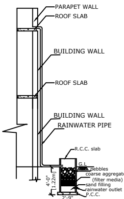
SEC. OF RAIN WATER HARVEST
