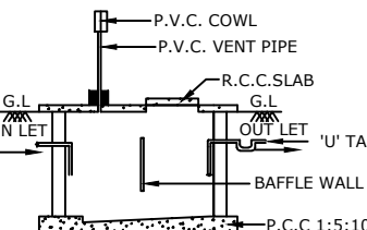
SEC. OF SEPTIC TANK
