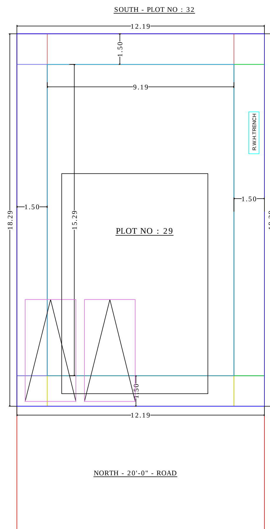
SITE PLAN
