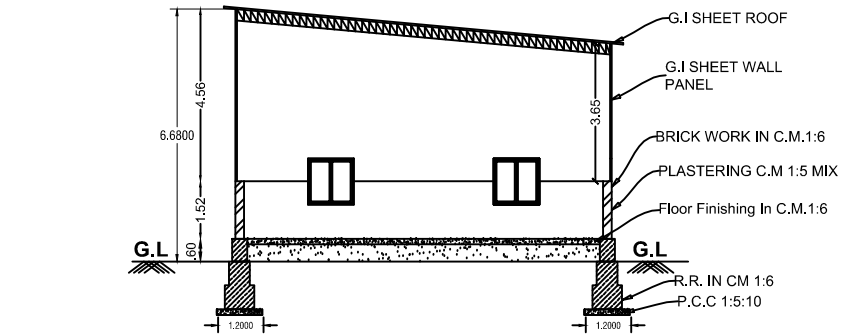
SECTION ON-"AB"
