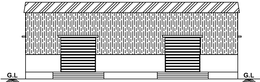
FRONT ELEVATION
