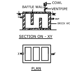
SEPTICTANK DETAILS NOT TO SCALE
