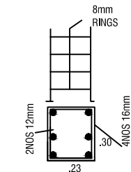
COLUMN DETAILS (NOT TO SCALE)
