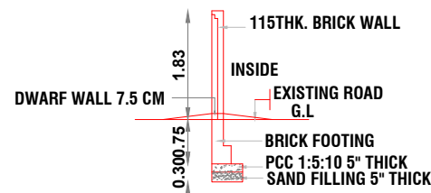
SECTION OF COMPOUND WALL
