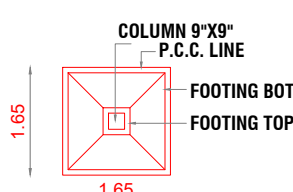
PLAN OF FOOTING
