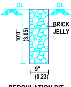
PERCOLATION PIT
