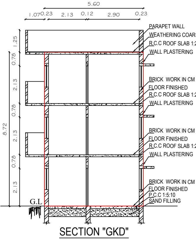
SECTION "GKD"
