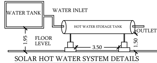
SOLAR HOT WATER SYSTEM DETAILS
