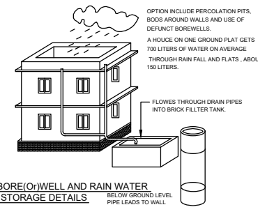
RAINWATER HARVESTING SCALE 1:50
