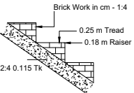
STAIR CASE DETAILS (Scale 1:1)
