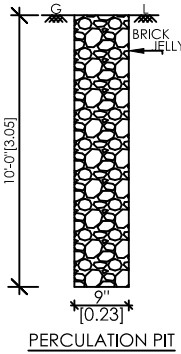
PERCOLATION PIT
