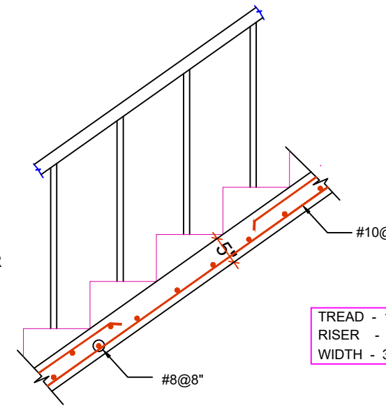
StairCase Detail
