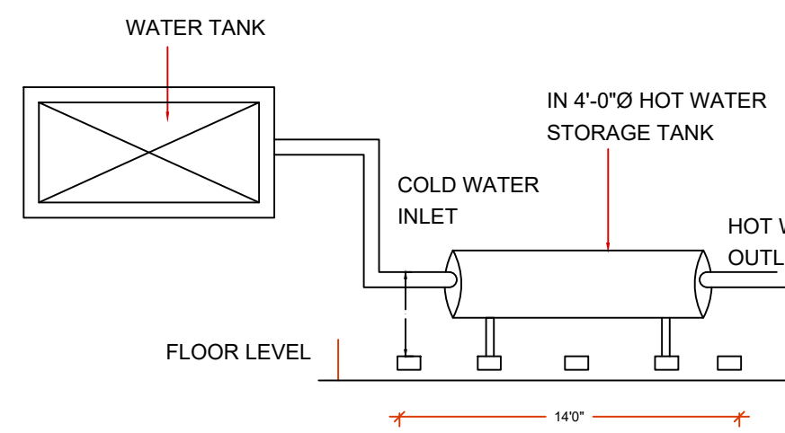
Solar Waterheater Detail
