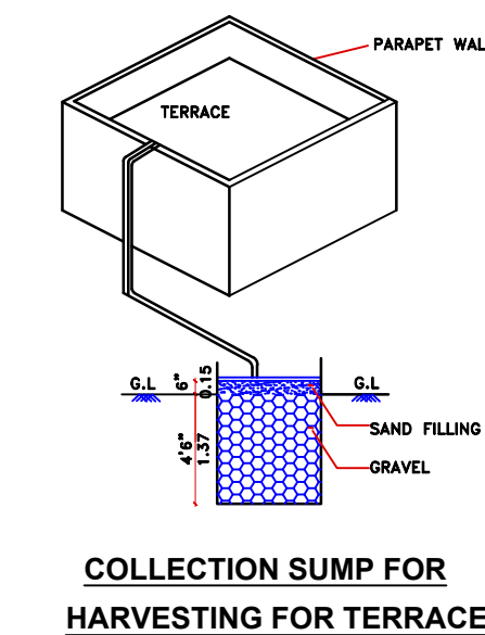
HARVESTING FOR TERRACE
