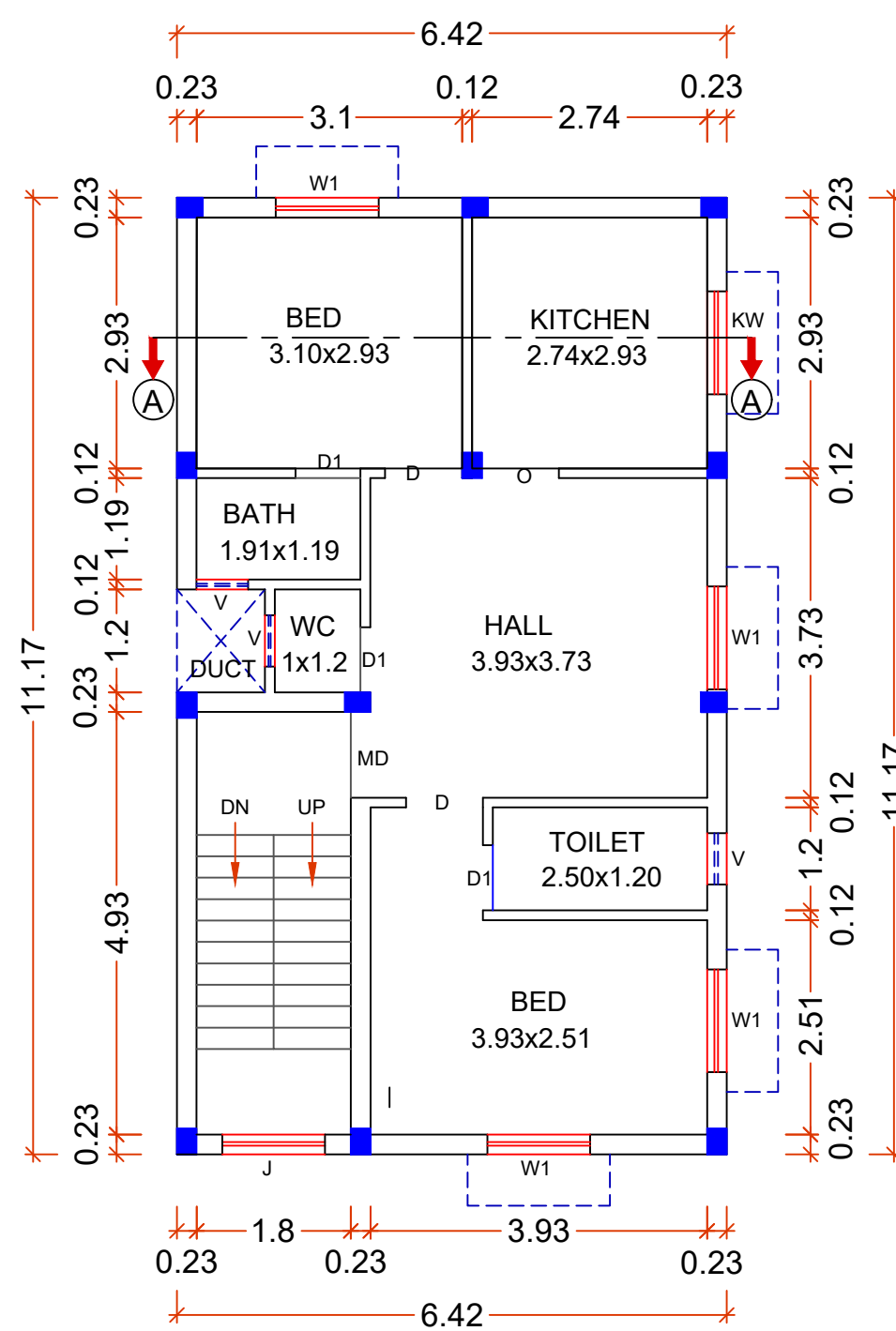
TYPICAL FLOOR PLAN ( FIRST & SECOND ) ( PROPOSED )
