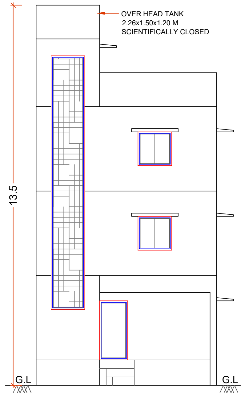
ELEVATION ( PROPOSED )
