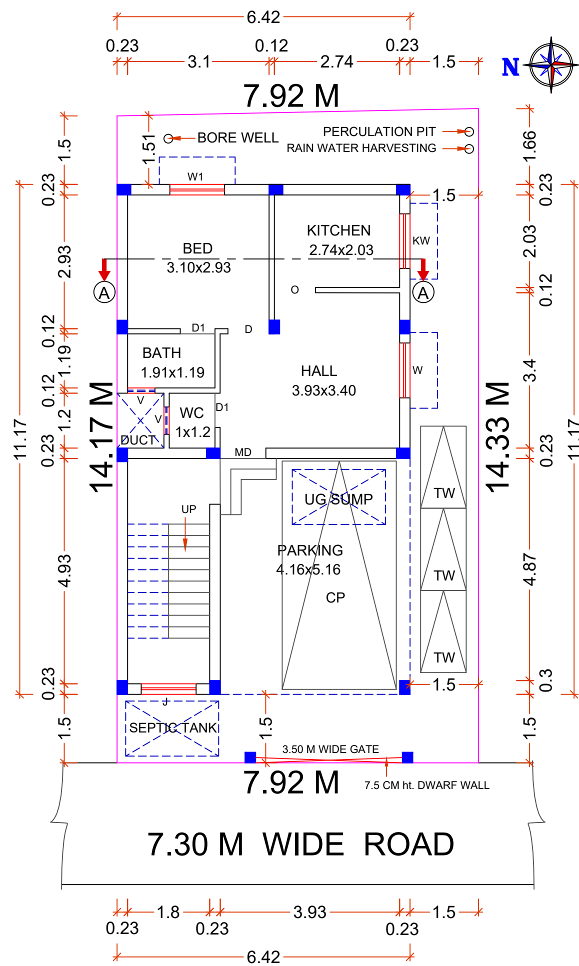
SITE CUM GROUND FLOOR PLAN
