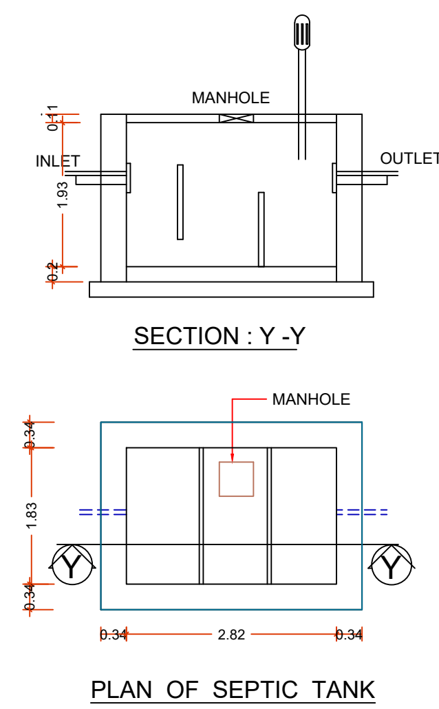
PLAN OF SEPTIC TANK
