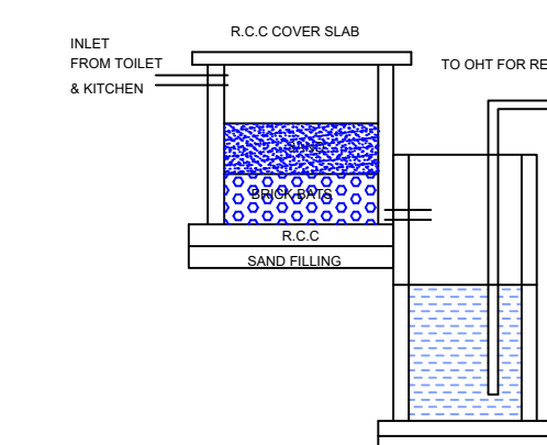
DETAILS OF RECYCLING OF WASTE WATER
