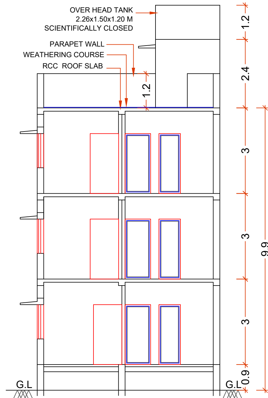
SECTION ON A - A ( PROPOSED )
