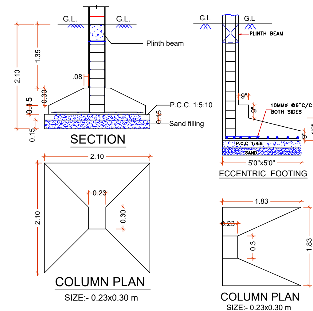
TYPICAL FOUNDATION DETAIL
