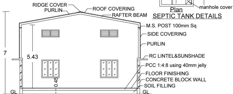
SECTION AT A-A
