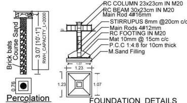
FOUNDATION DETAILS
