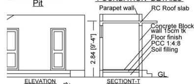
FOUNDATION DETAILS
