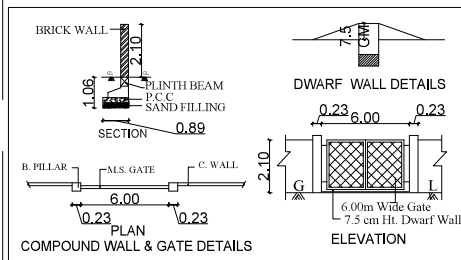
COMPOUND WALL & GATE DETAILS
