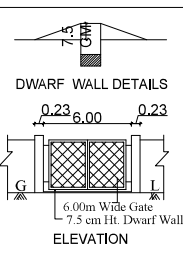
DWARF WALL DETAILS
