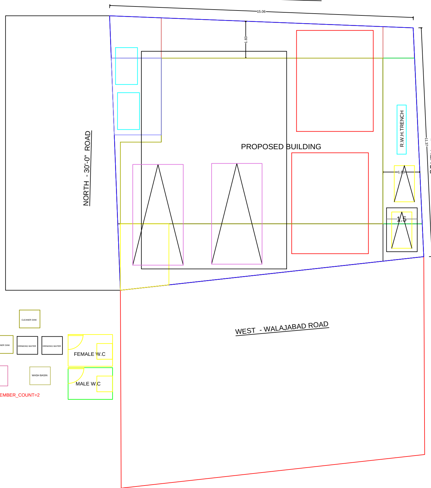
SITE PLAN
