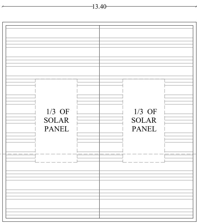
TERRACE FLOOR
