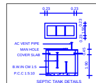
SEPTIC TANK DETAIL
