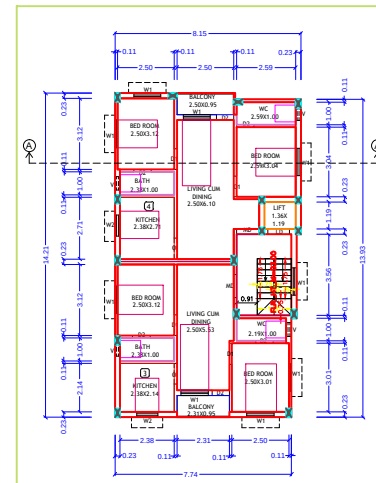
SECOND FLOOR PLAN (PROPOSED)
