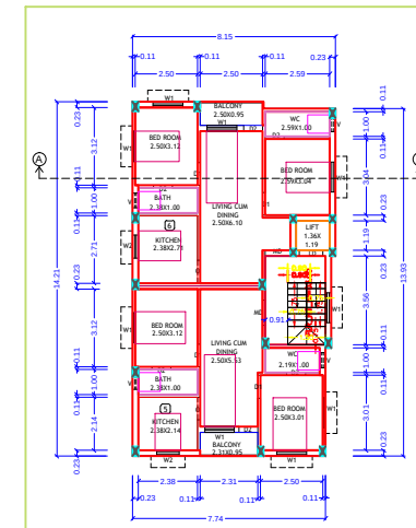
THIRD FLOOR PLAN (PROPOSED)
