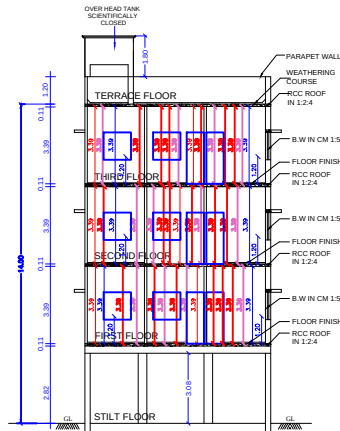
SECTION ON 'AA' (PROPOSED)
