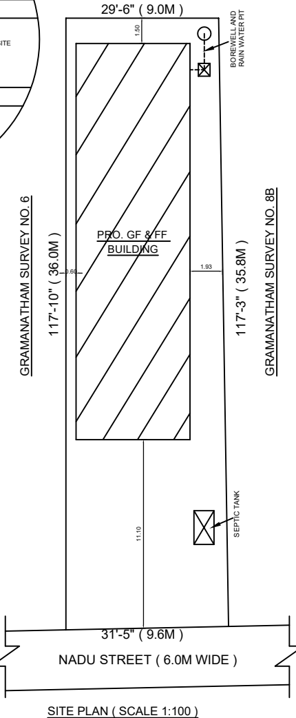
MR. KARTHIKEYAN'S PLOT
