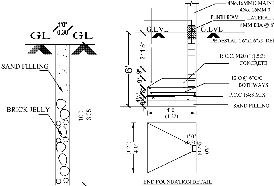
PERCOLATION PIT
