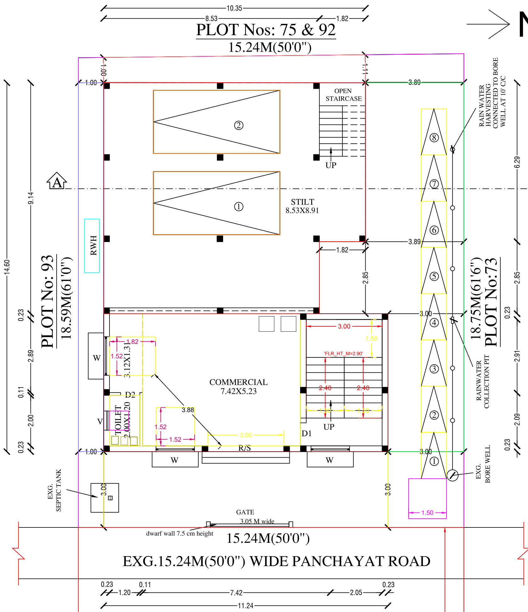
SITE PLAN CUM STILT & GROUND FLOOR PLAN (EXG. & PRO)(COM.)
