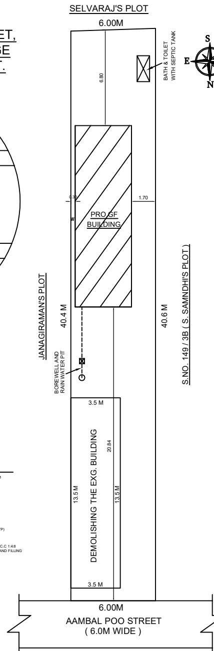
RAIN WATER HARVESTING SYSTEM
