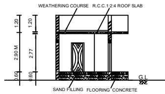
SECTION ON "MS"
