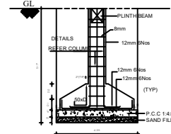
FOUNDATION DETAILS
