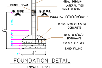
FOUNDATION DETAIL (SCALE: 1:50)
