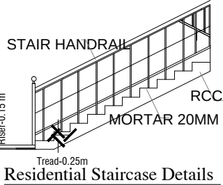
Residential Staircase Details
