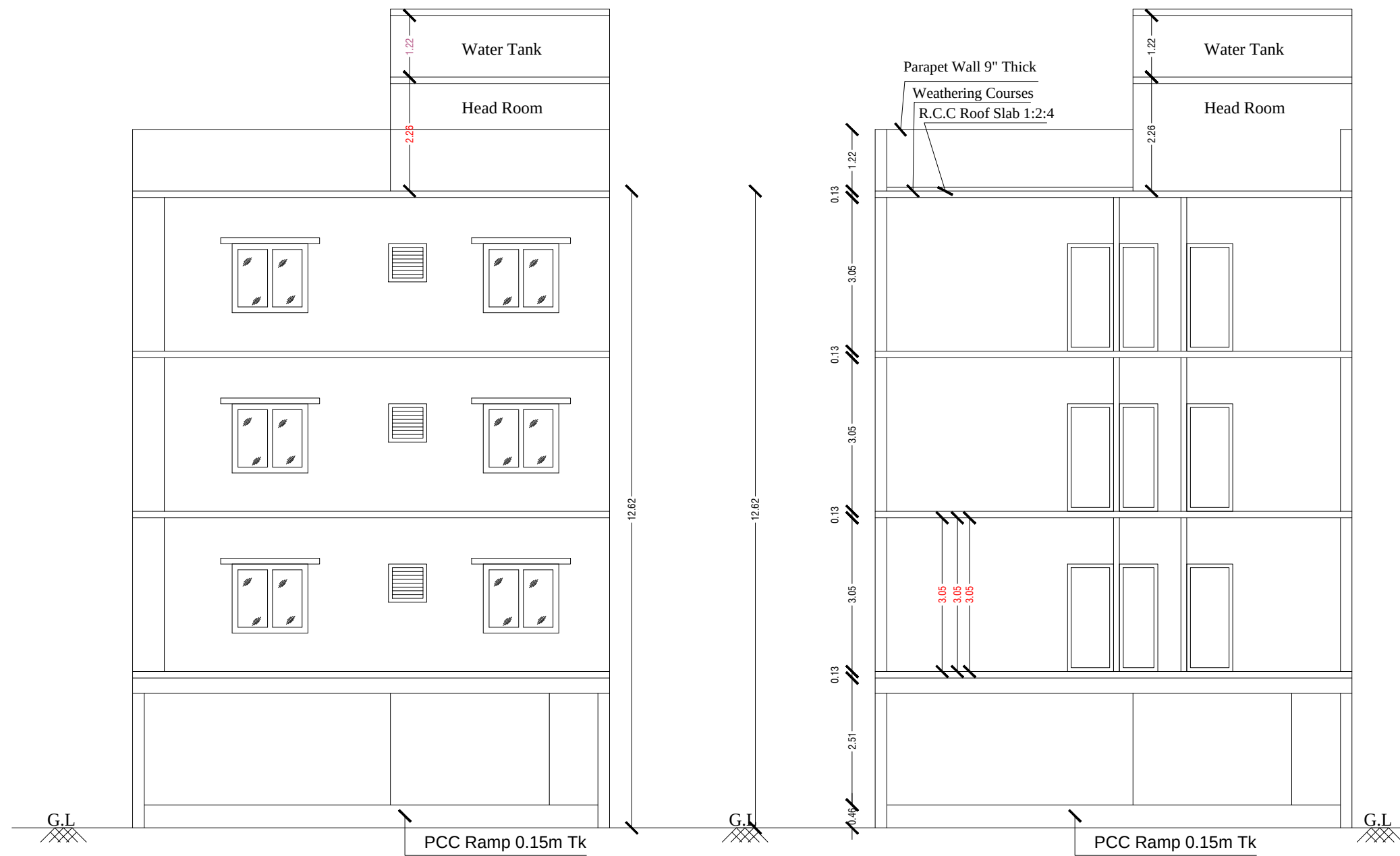
CROSS SECTION ON AB
