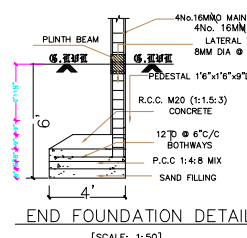
END FOUNDATION DETAIL (SCALE: 1:50)
