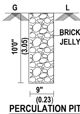
PERCULATION PIT
