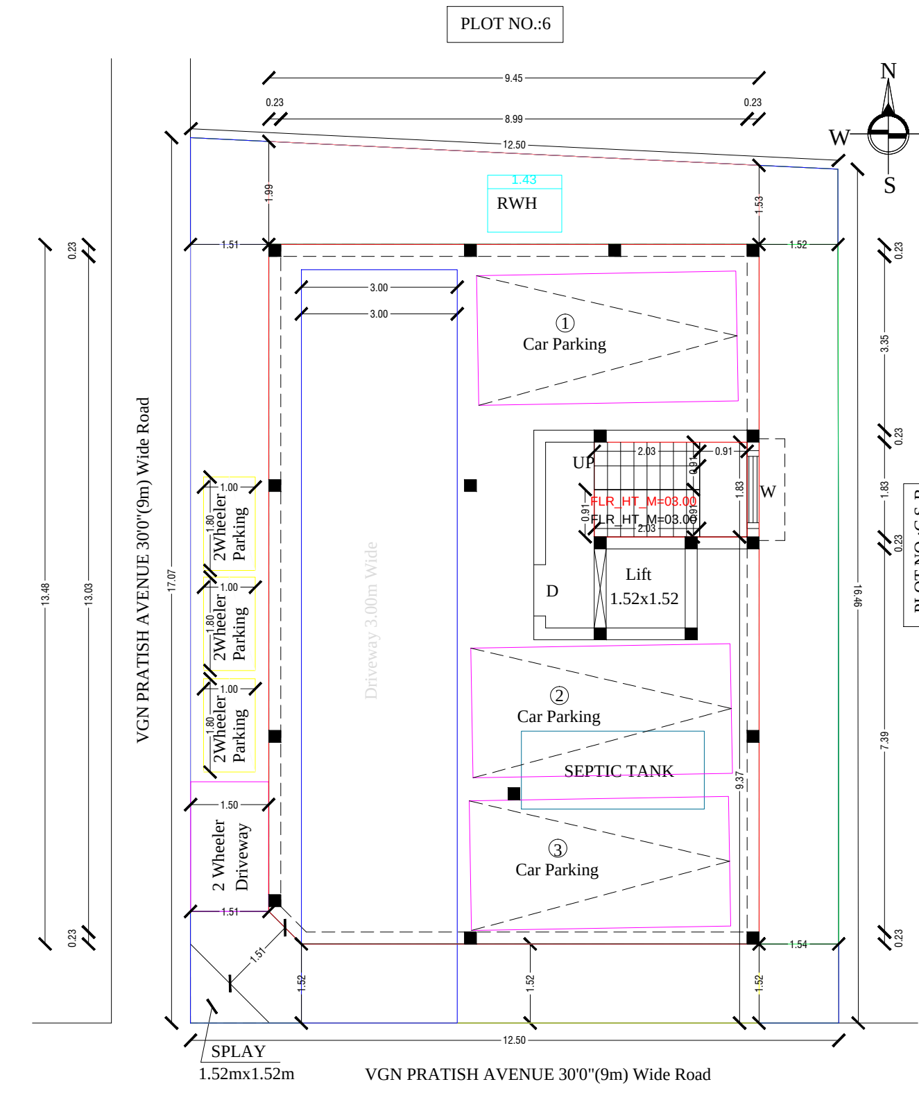
FE CUM STILT FLOOR PLAN
