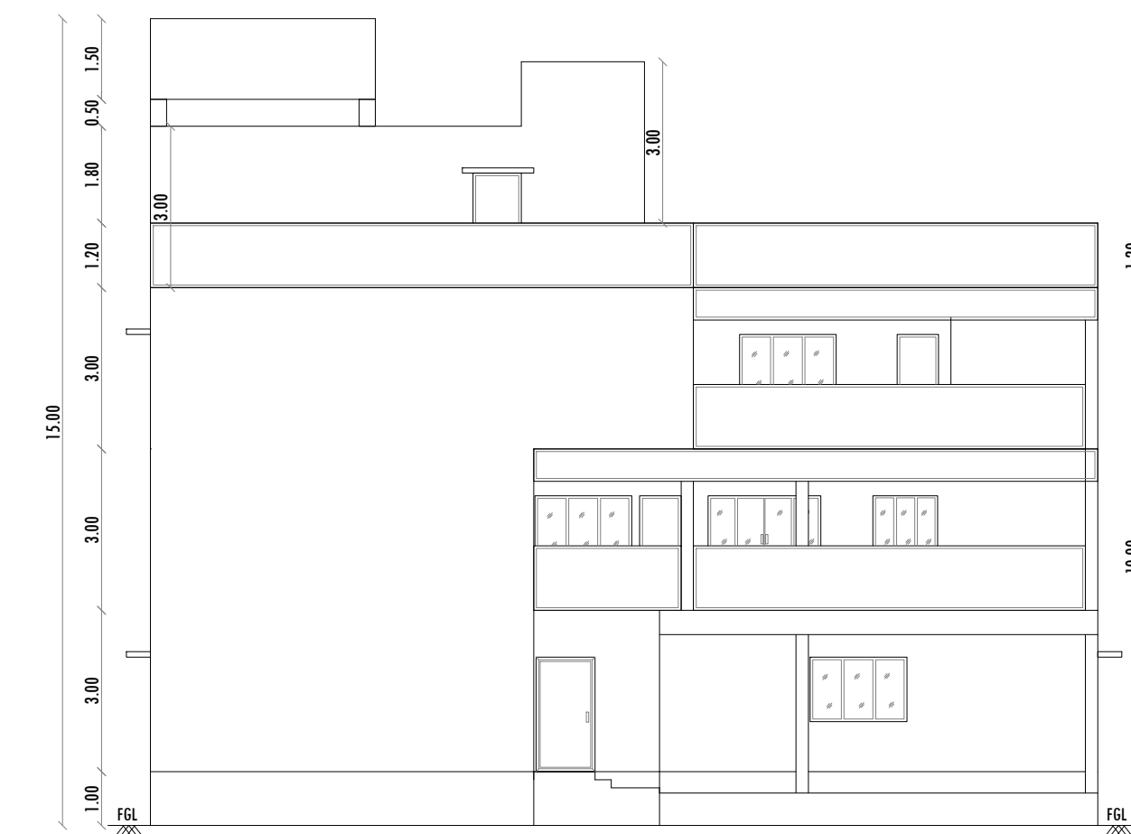
FRONT ELEVATION (PROPOSED)
