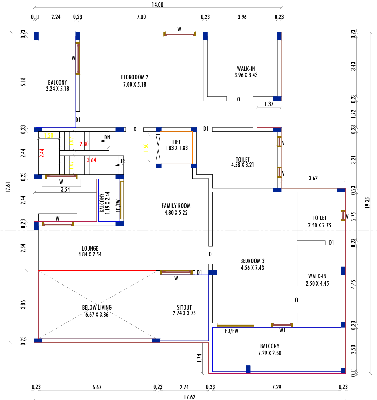
FIRST FLOOR PLAN (PROPOSED)
