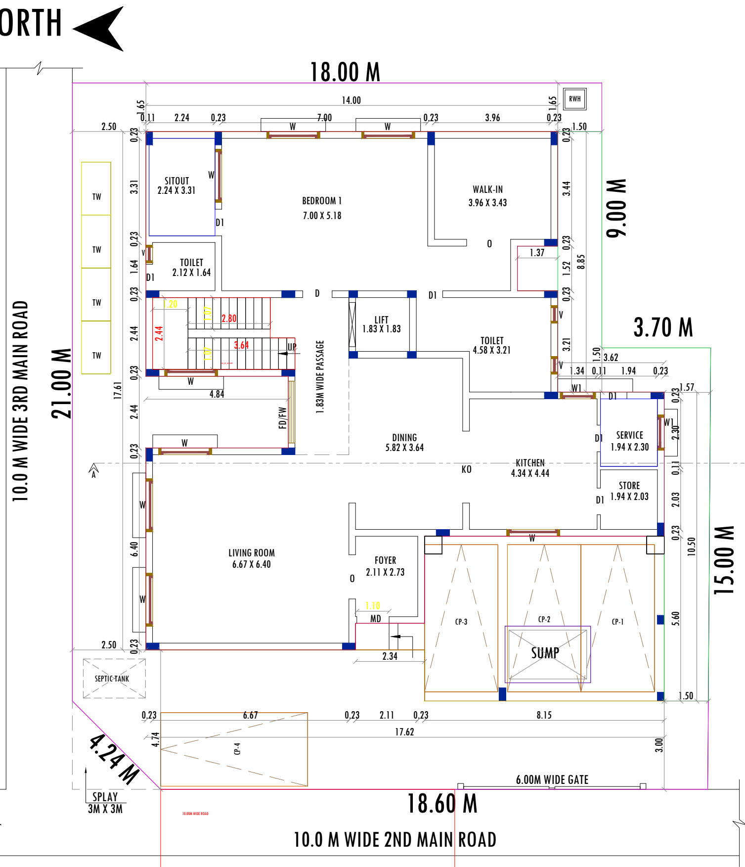
SITE CUM GROUND FLOOR PLAN (PROPOSED)
