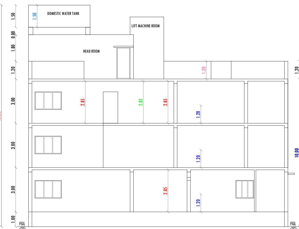
SECTION ON 'A-A' (PROPOSED)
