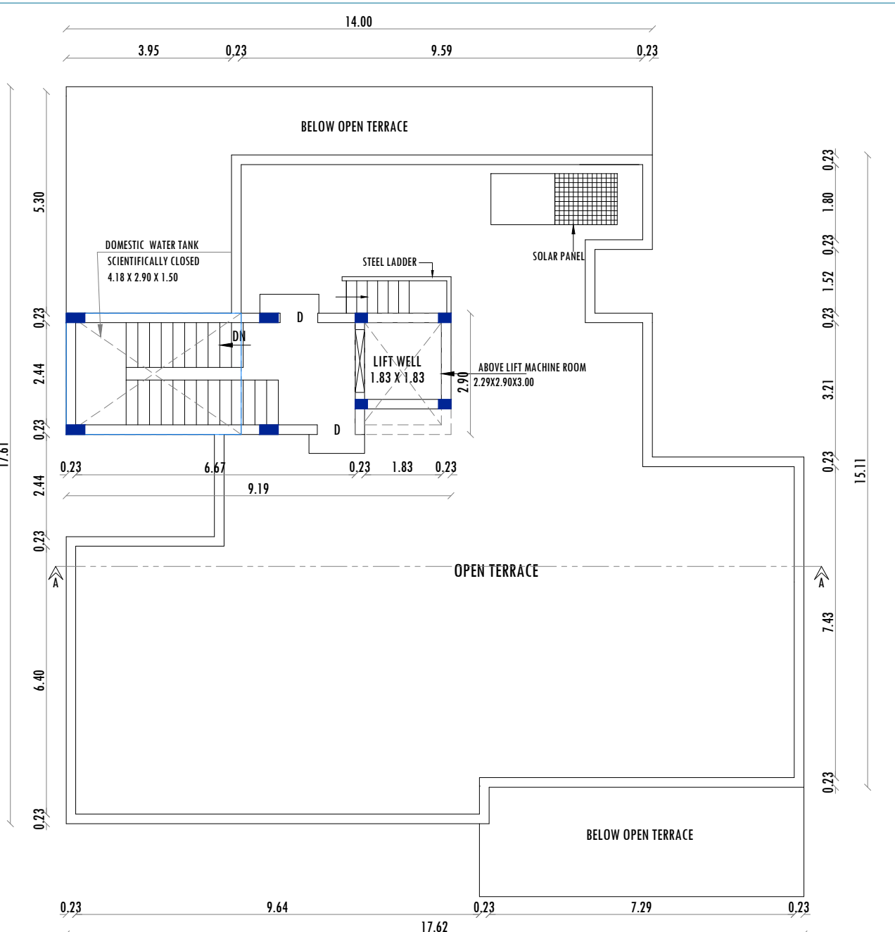
TERRACE FLOOR PLAN (PROPOSED)
