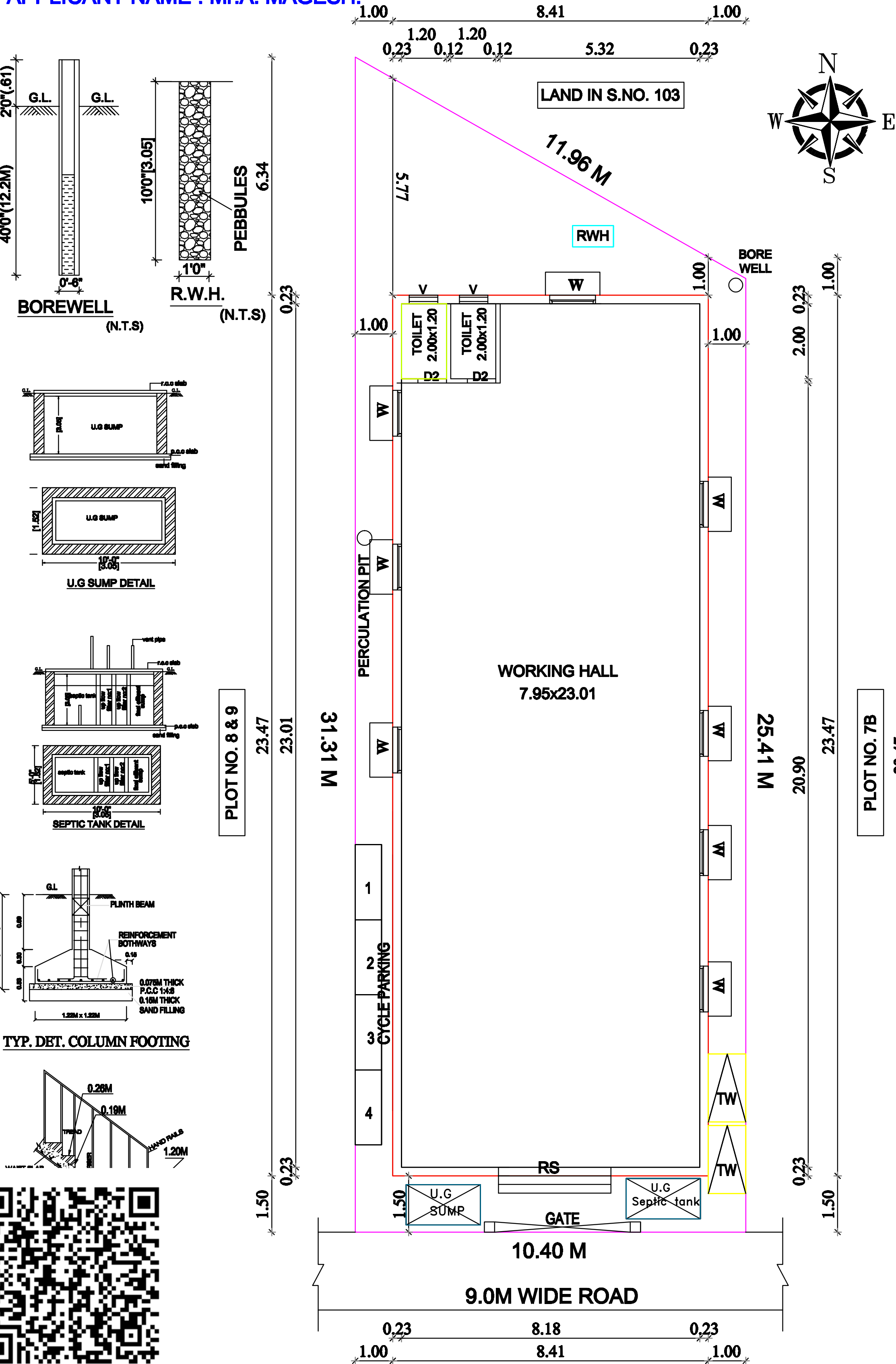
SITE CUM GROUND FLOOR PLAN PROPOSED
