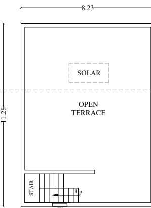
TERRACE FLOOR
