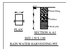
RAIN WATER HARVESTING P.T.
