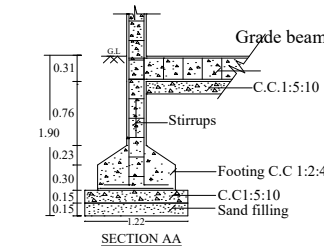
FOUNDATION DETAILS
