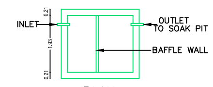
PLAN SEPTIC TANK
