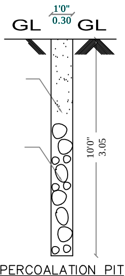
PERCOLATION PIT
