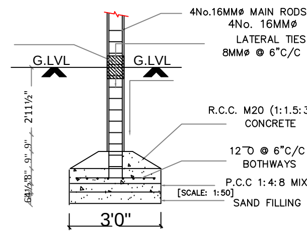
FOUNDATION DETAIL
