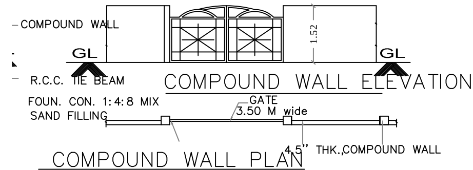
COMPOUND WALL PLAN
