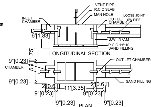
SEPTIC TANK:
