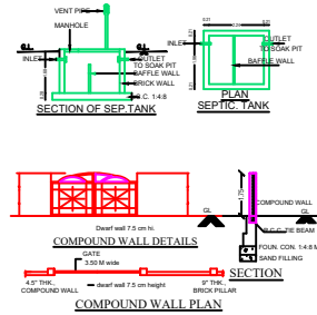
COMPOUND WALL PLAN
