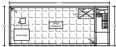
TERRACE FLOOR PLAN
