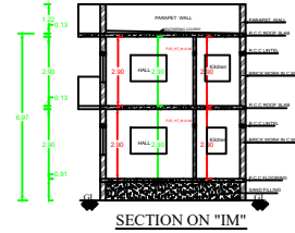
SECTION ON "IM"
