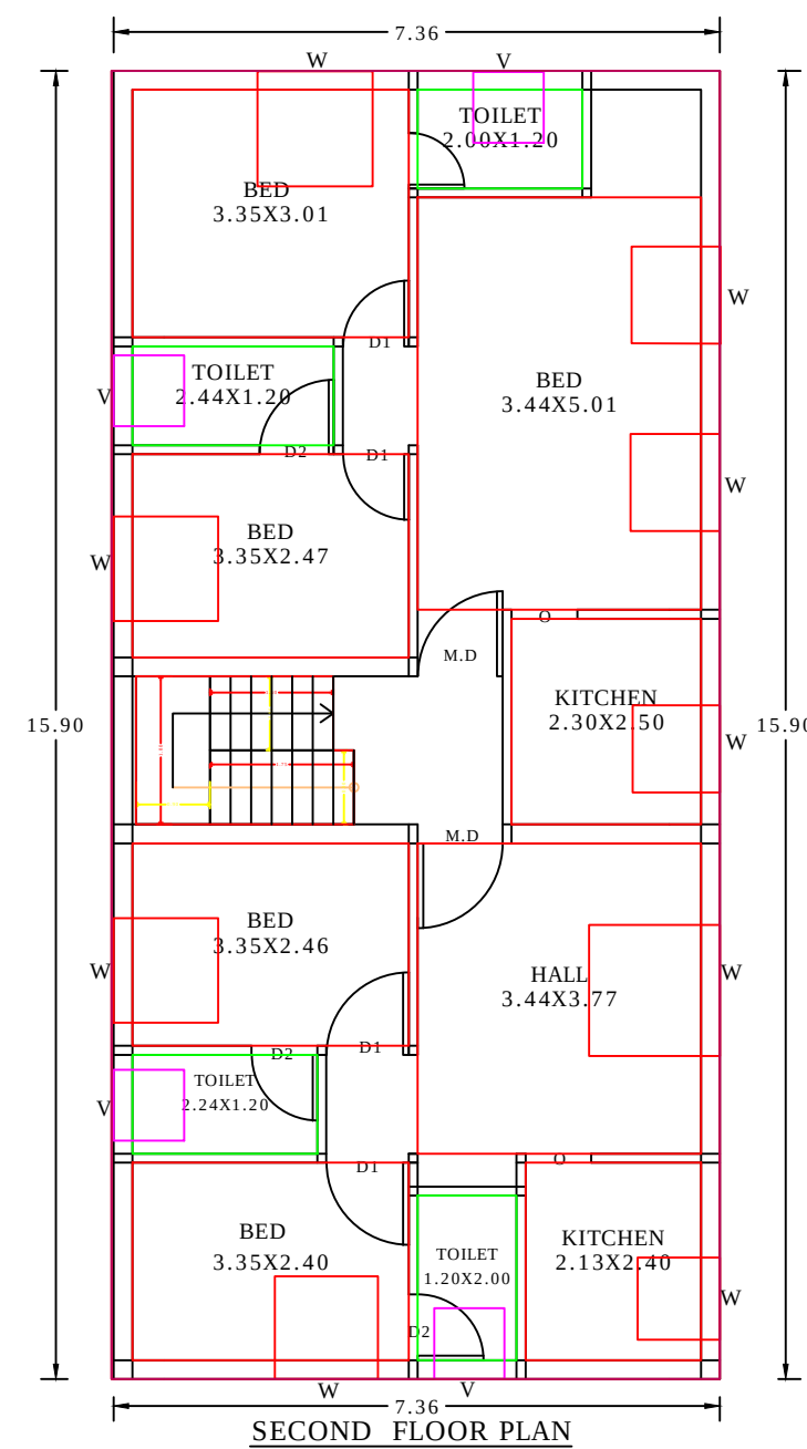
7.36 SECOND FLOOR PLAN
