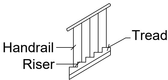
STAIRCASE DETAIL
