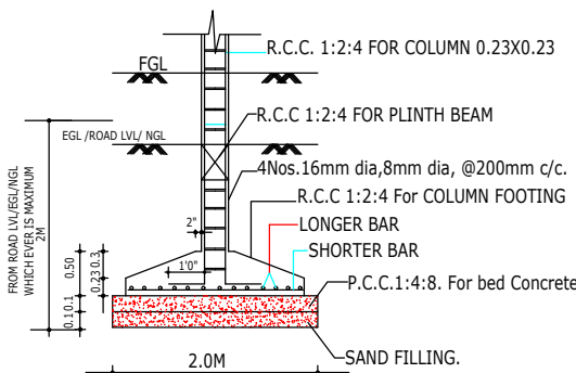
FOUNDATION DETAIL
