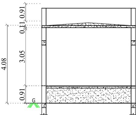
SECTION ON "SC"
