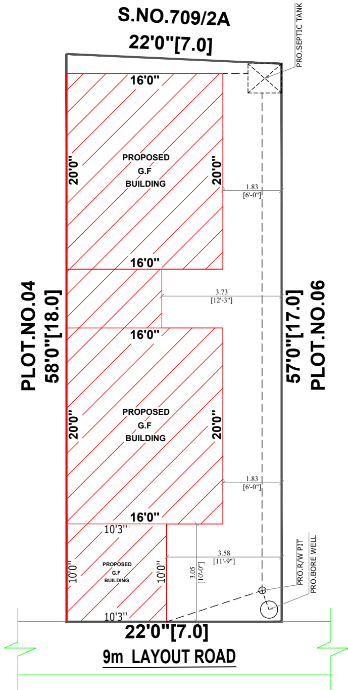
SITE PLAN SCALE: 1 INCH = 8 FEET
