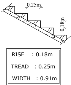
STAIRS DETAILS
