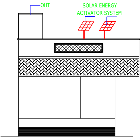
FRONT ELEVATION
