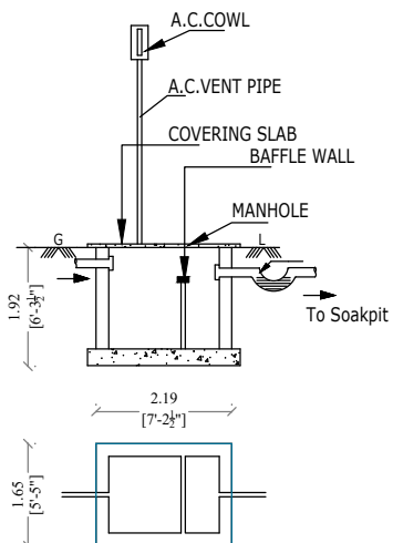
SEPTIC TANK
