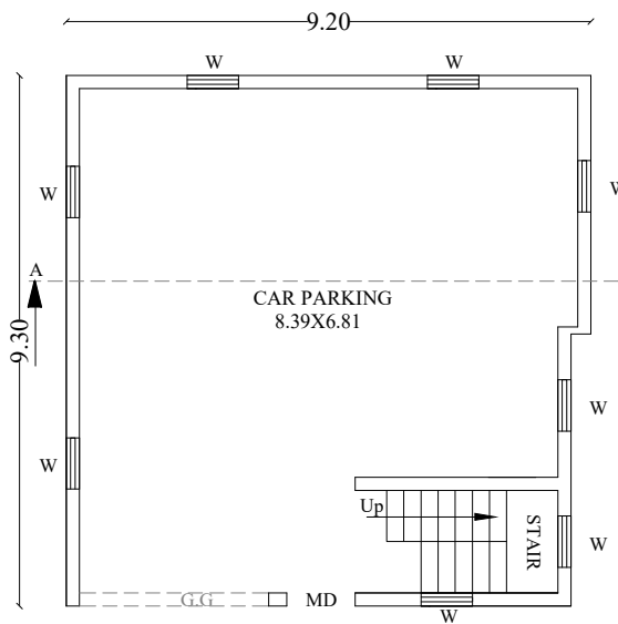
STILT FLOOR
