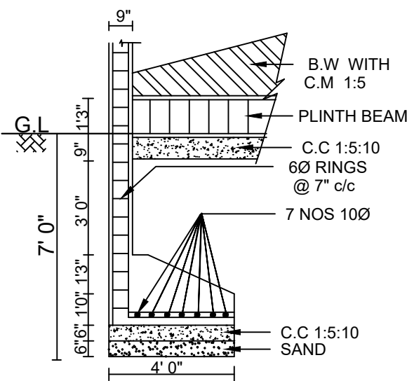
FOUNDATION DETAILS
