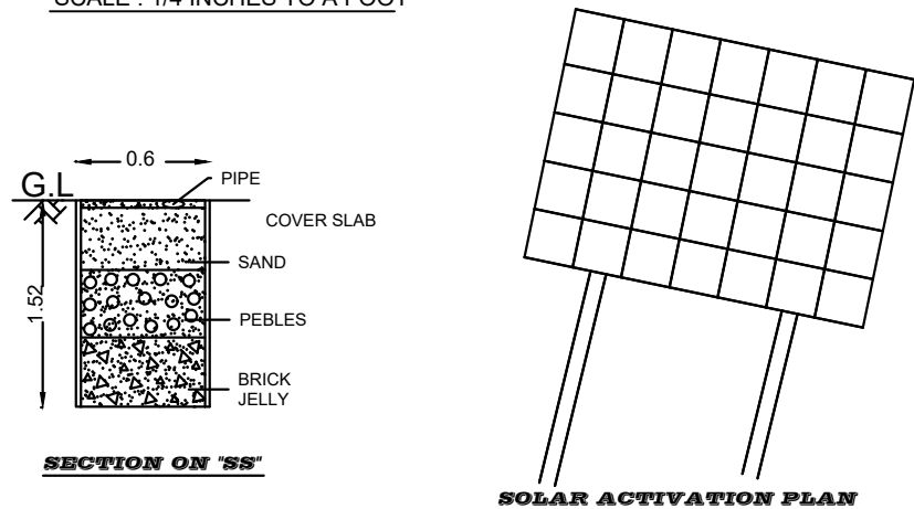
SOLAR ACTIVATION PLAN
