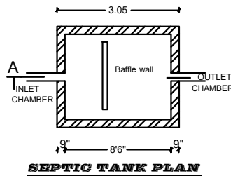
SEPTIC TANK PLAN
