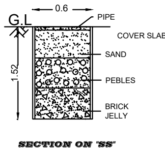
SECTION ON 'SS'
