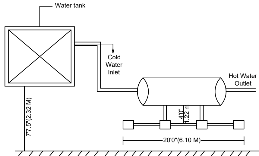
SOLAR HOT WATER SYSTEM
