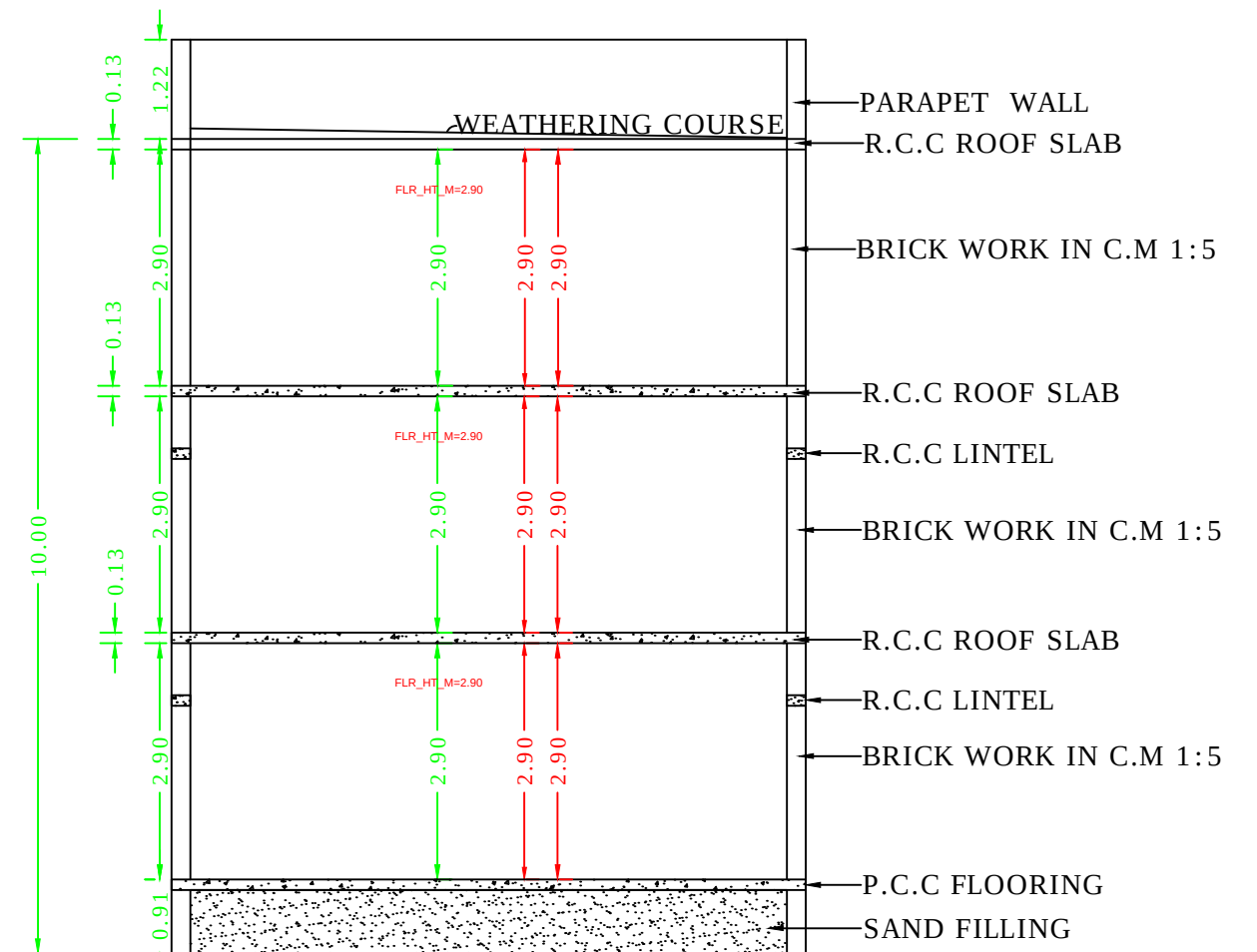
SECTION
