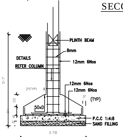
FOUNDATION DETAILS
