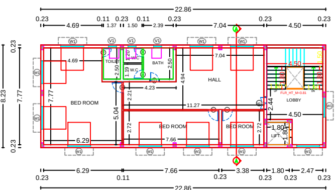
SECOND FLOOR PLAN (PROPOSED)
