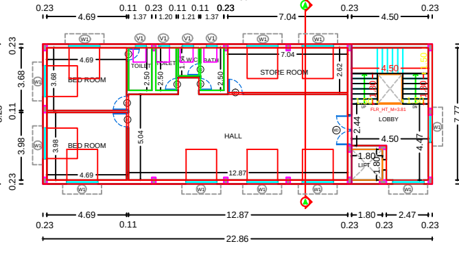
FIRST FLOOR PLAN (PROPOSED)
