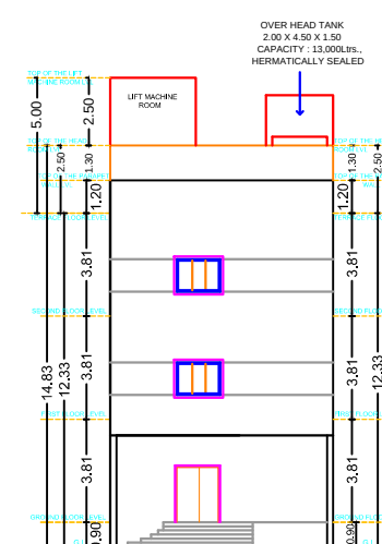
FRONT ELEVATION
