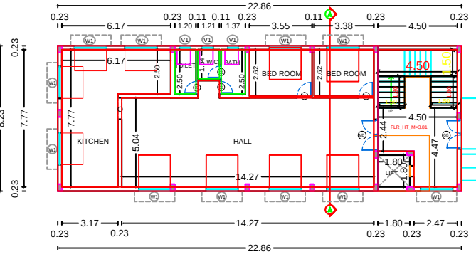
GROUND FLOOR PLAN (PROPOSED)
