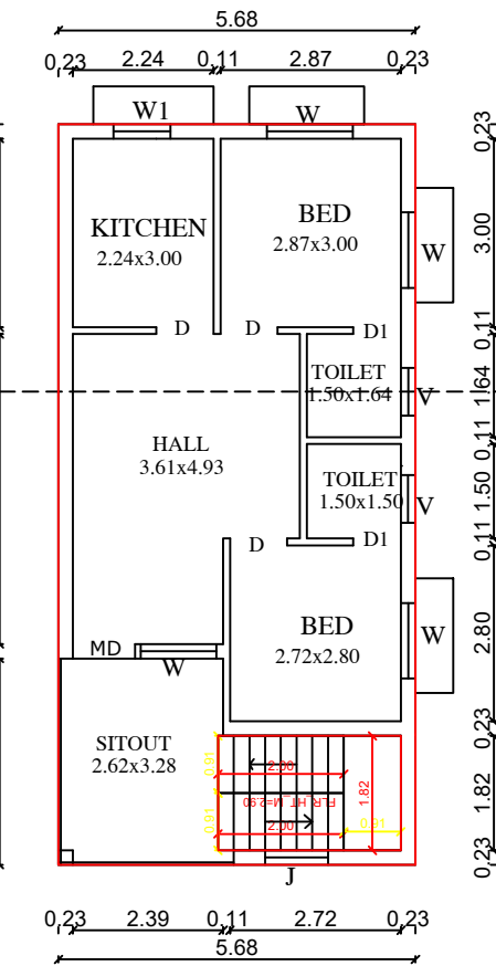
EXG FIRST FLOOR PLAN
