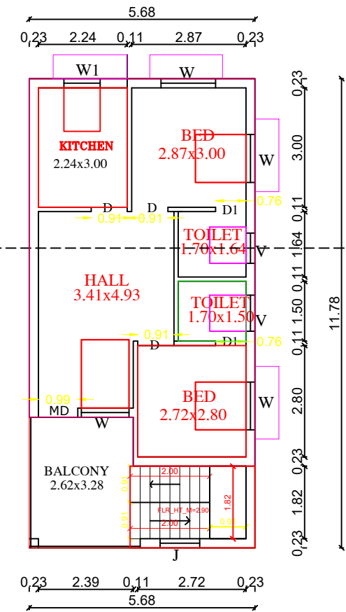
PRO. SECOND FLOOR PLAN
