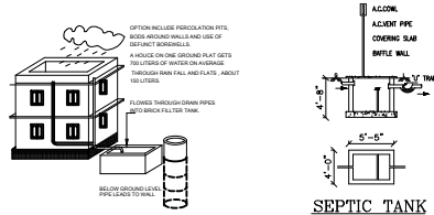
SEPTIC TANK
