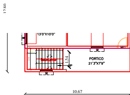
PROPOSED GROUND FLOOR PLAN
