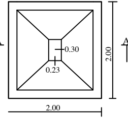
RAFT FOUNDATION PLAN SCALE : NTS
