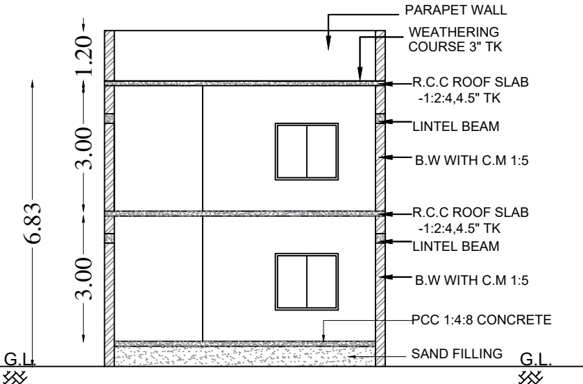
SECTION AT "XX"
