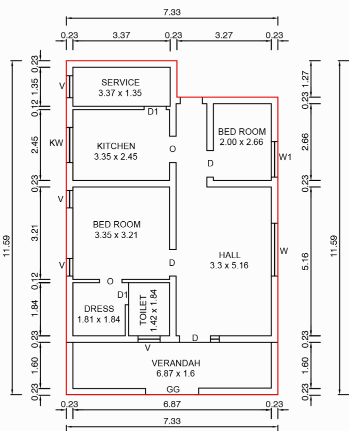
EXISTING GROUND FLOOR TO BE DEMOLITION
