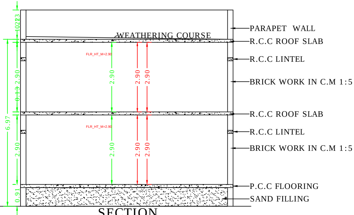
SECTION
