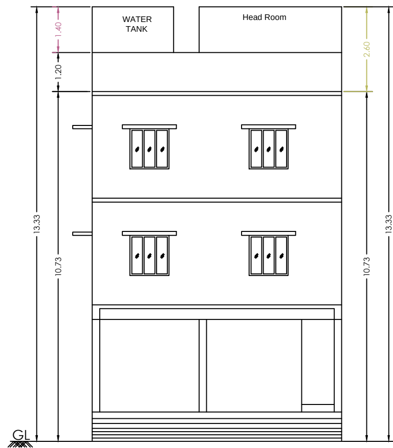
FRONT ELEVATION.
