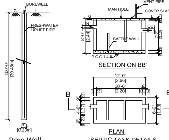
Bore Well SEPTIC TANK DETAILS
