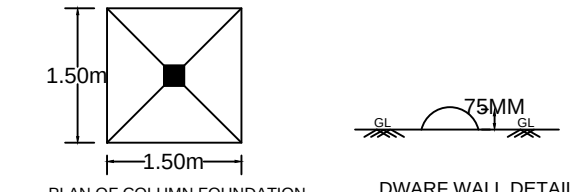
PLAN OF COLUMN FOUNDATION DWARF WALL DETAIL
