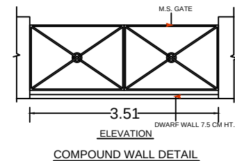
COMPOUND WALL DETAIL SCALE = 1 : 50
