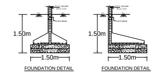
FOUNDATION DETAIL
