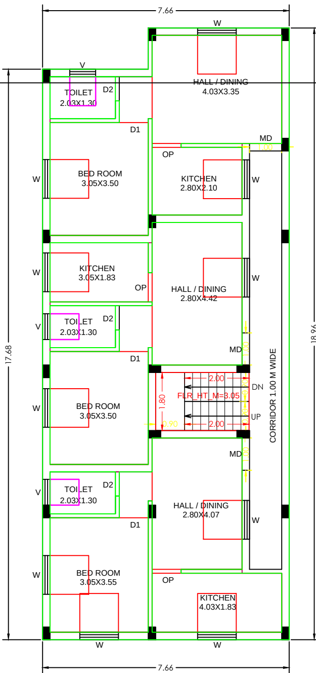
TYPICAL FLOOR PLAN=1.2 TYPICAL_FLOOR_PLAN=1.2
