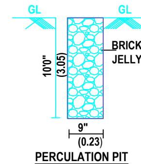
PERCULATION PIT
