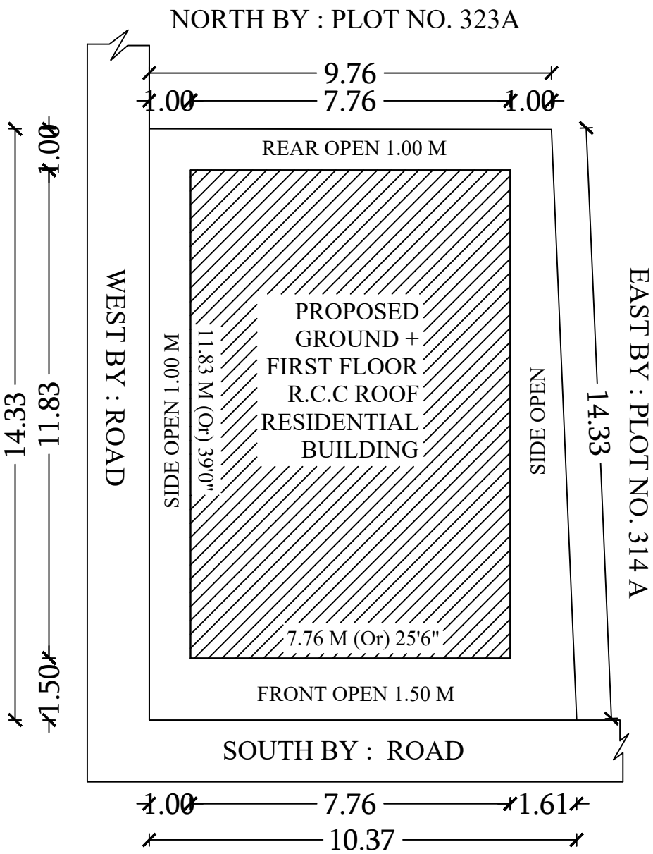
SITE PLAN
