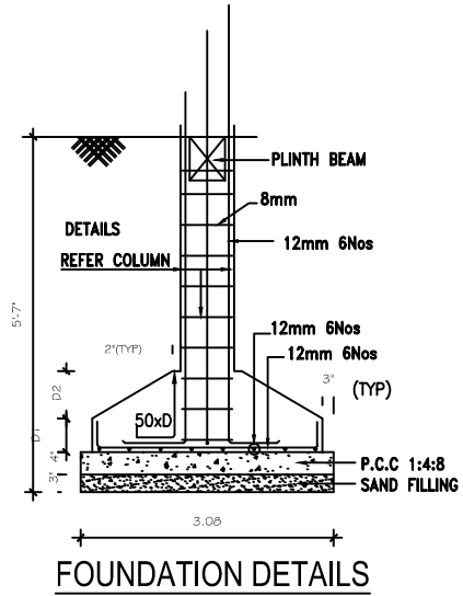
FOUNDATION DETAILS
