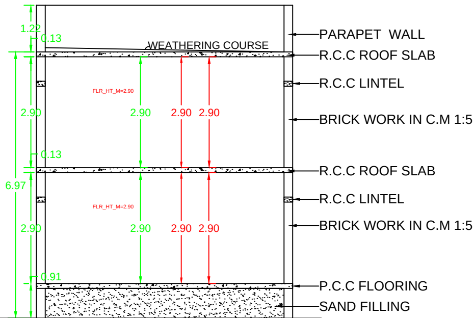
SECTION
