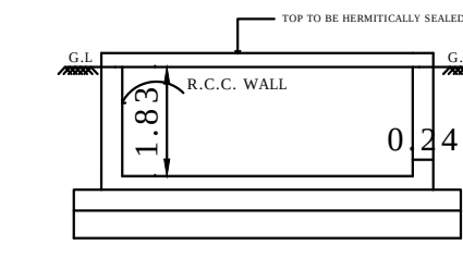
RWHT SECTION (SAMPLE) RWHT_CAPACITY_L=5000LTRS
