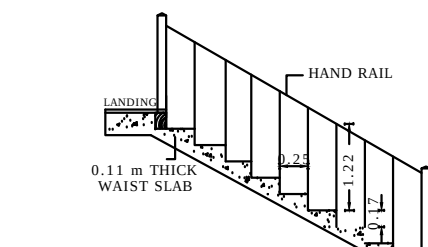
STAIRCASE DETAIL
