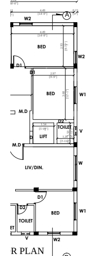
R PLAN
