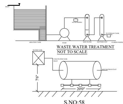
SOLOR HOT WATER SYSTEM DETAILS
