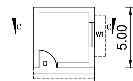
SECURITY OFFICE FLOOR PLAN
