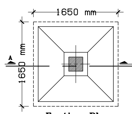
Footing Plan
