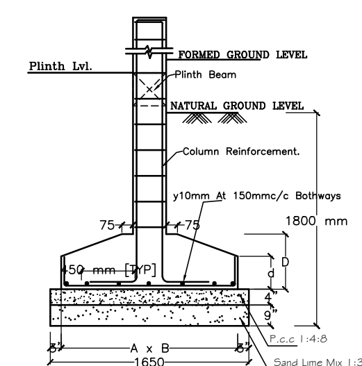
Footing Section
