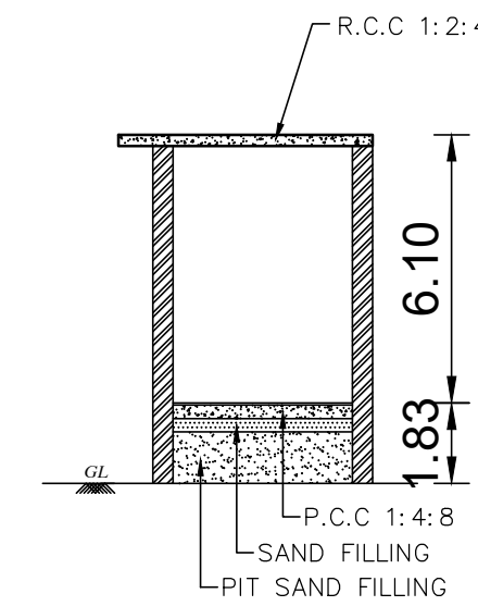
SECTION ON 'CC'
