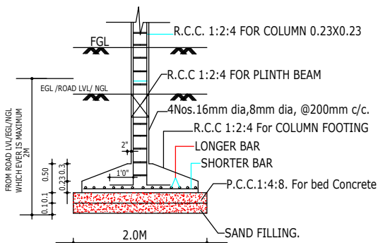
FOUNDATION DETAIL
