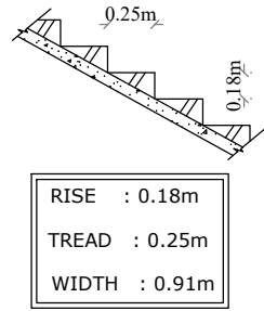
STAIRS DETAILS
